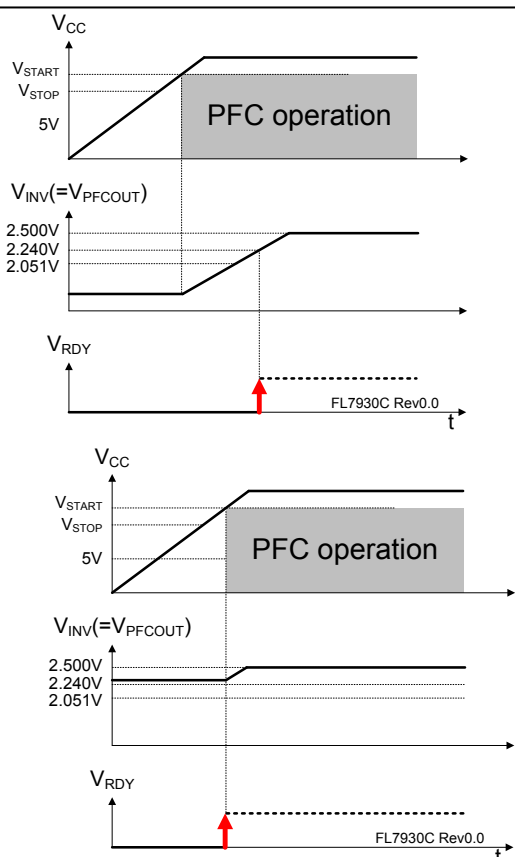
Figure 25. Two Cases of RDY Triggered HIGH
