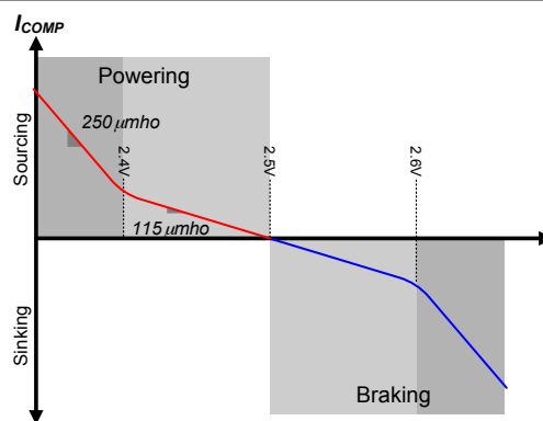
Figure 35. Gain Characteristic
