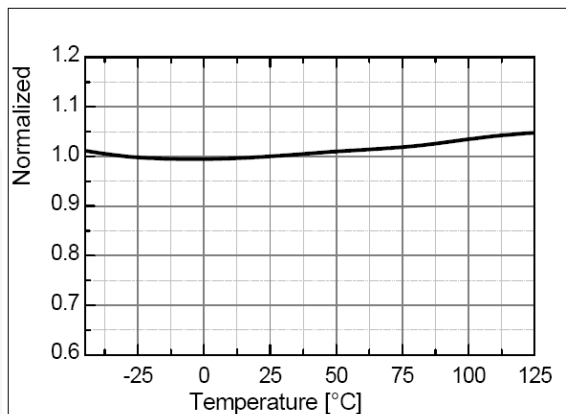
Figure 12. Maximum On-Time Program 1 (t ON,MAX1 ) vs. T A
