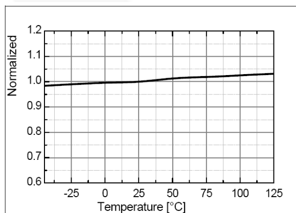
Figure 15. Input High Clamp Voltage (V CLAMPH ) vs. T A
