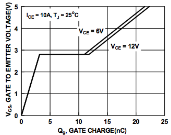
Figure 10. Gate Charge
