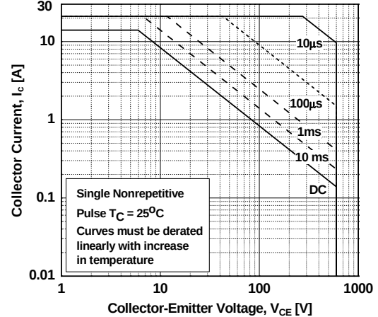
Figure 10. SOA Characteristics
