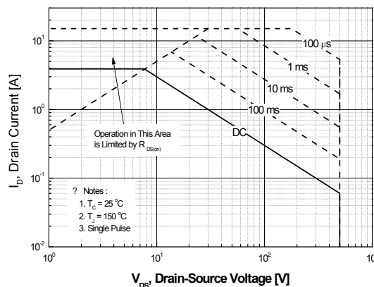
Figure 8. Maximum Safe Operating Area vs. Case Temperature-FDPF5N50NZU
