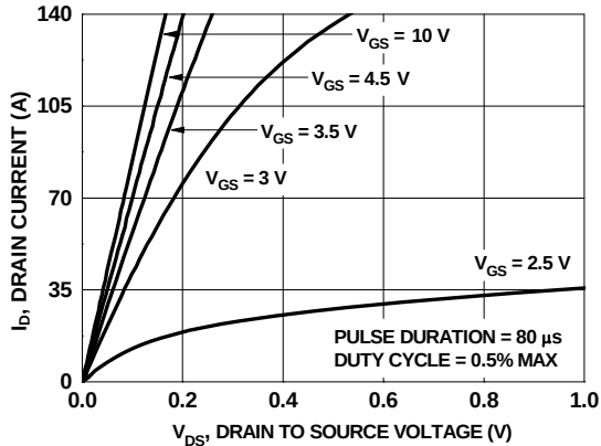
Figure 14. On-Region Characteristics
