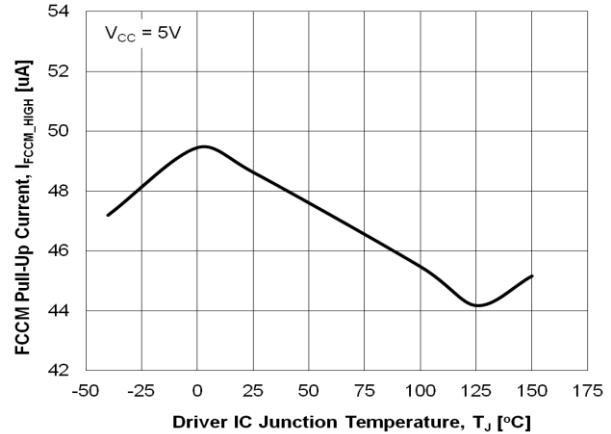
Figure 21. FCCM Pull-Up Current vs. Temperature
