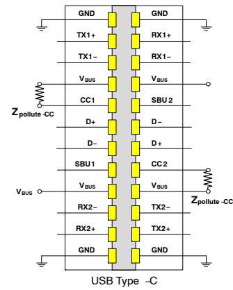
Figure 39. CC1/CC2 Short-circuited with Impedance
