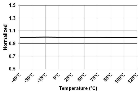
Figure 26. V_{IN} UVP Enable Voltage at 12 V ( V_{IN-UVLP-L-12V} ) vs. Temperature
