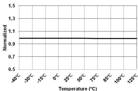
Figure 27. V_{IN} UVP Disable Voltage at 12 V ( V_{IN-UVLP-H-12V} ) vs. Temperature
