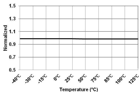
Figure 24. V_{IN} UVP Enable Voltage at 9 V ( V_{IN-UVLP-L-9V} ) vs. Temperature
