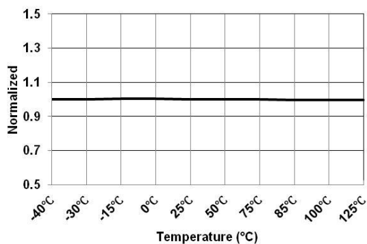
Figure 25. V_{IN} UVP Disable Voltage at 9 V ( V_{IN-UVLP-H-9V} ) vs. Temperature
