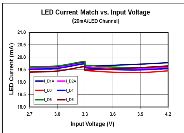
Figure 5. LED Current Match for all 6 LED Channels at I_{LED}=20\text{ mA}
