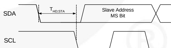
Figure 20. Start Bit
