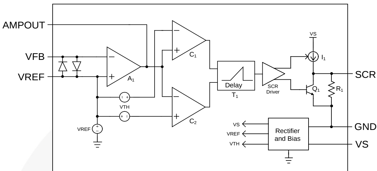
Figure 1. Block Diagram
