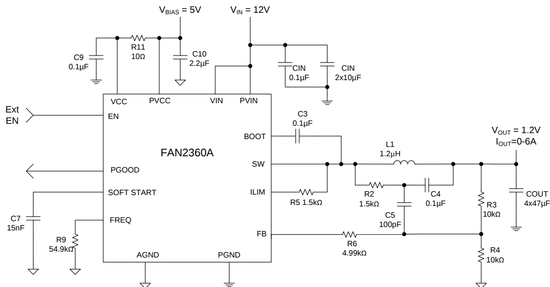
Figure 1. Typical Application
