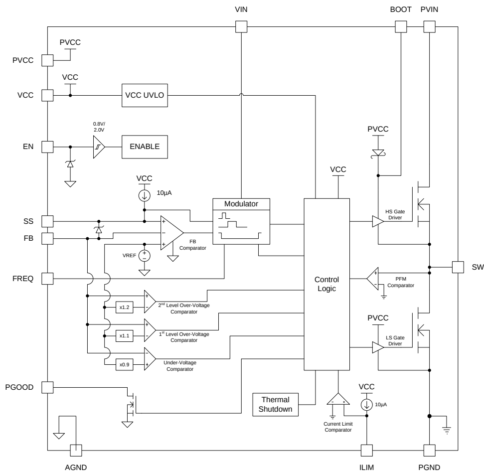
Figure 2. Block Diagram
