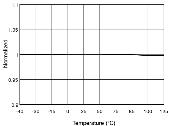
Figure 5. Turn-Off Threshold Voltage ( V_{DD-OFF} ) vs. Temperature
