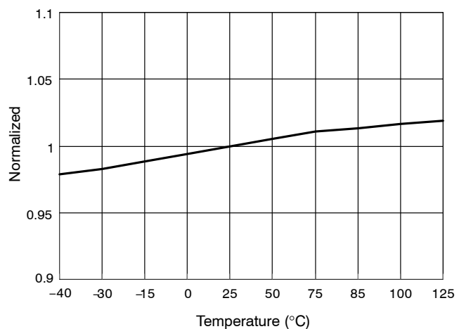
Figure 9. Minimum Blanking Frequency ( f_{BNK-MIN} ) vs. Temperature
