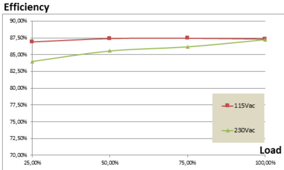
Figure 30. Board Efficiency
