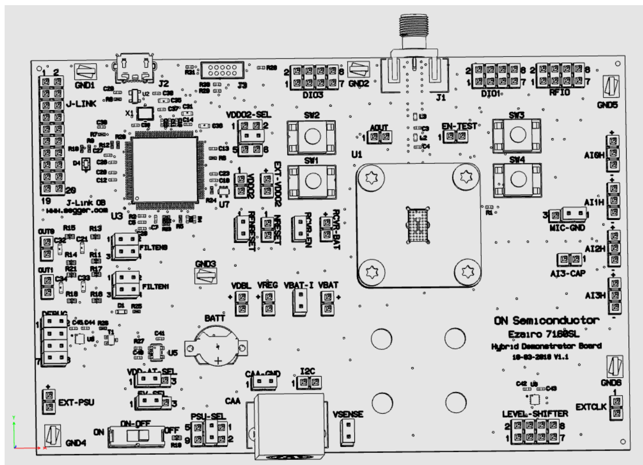
Figure 4. Three-Dimensional Line Drawing of the Board (Top View)
