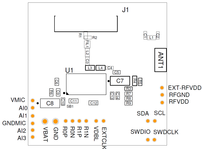
Figure 3. Daughterboard Circuit Location Block Diagram
