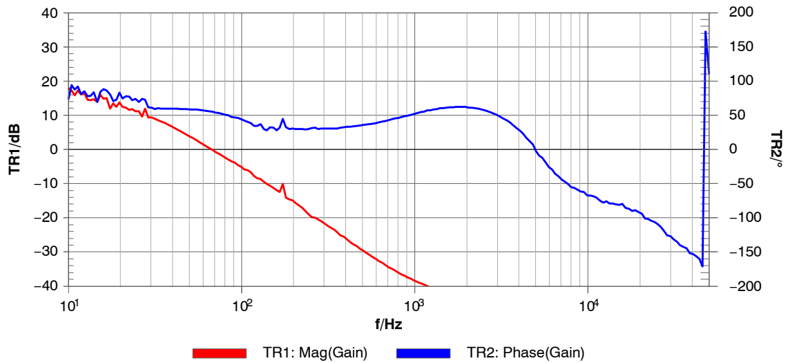
Figure 40. V_{IN} = 230\text{ V}_{AC} , I_{OUT} = 5.9\text{ A} , V_{OUT} = 10\text{ V}
