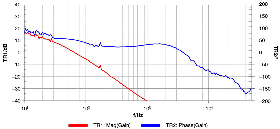
Figure 39. V_{IN} = 115\text{ V}_{AC} , I_{OUT} = 5.9\text{ A} , V_{OUT} = 10\text{ V}
