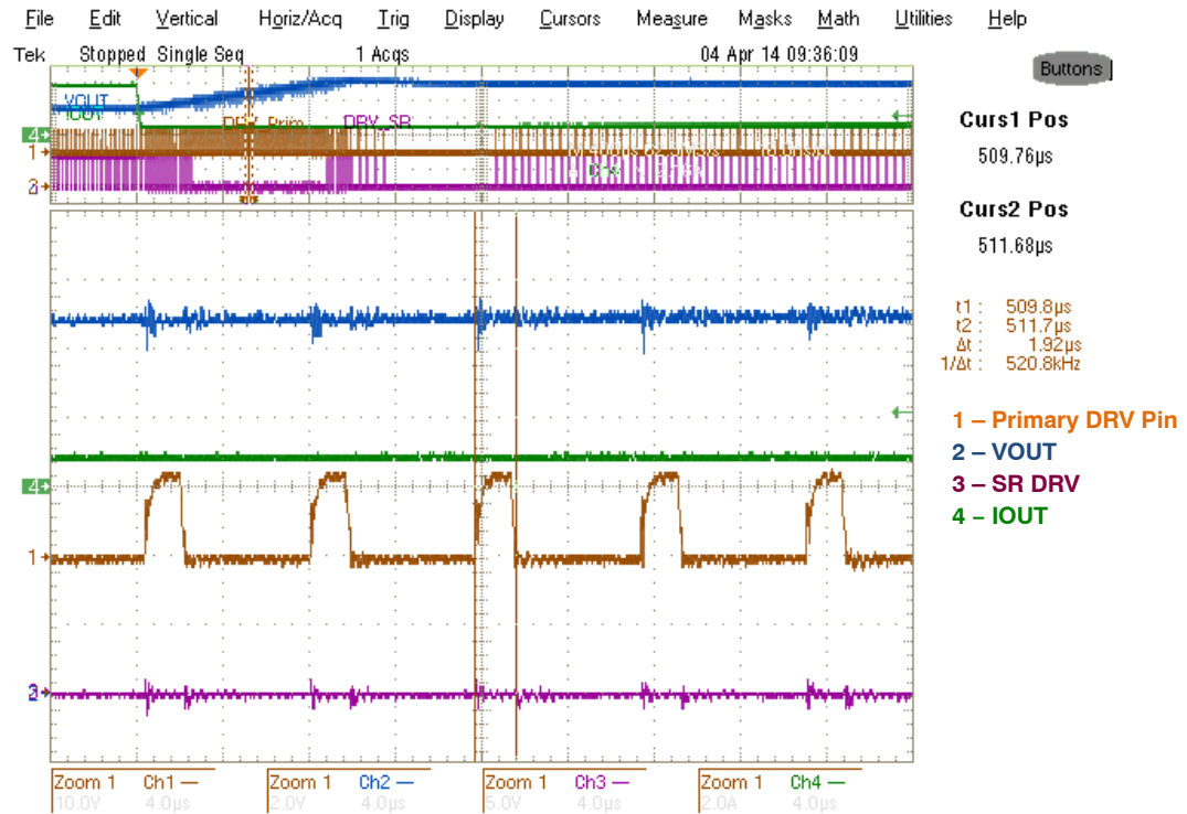
Figure 32. V_{IN} = 230 \text{ V}_{AC} , R_{OUT} = 1.5 \Omega to 10 \Omega – Detail Shows why SR is Not Turned On. It is Not Turned-on, because Primary On-time is Shorter than Secondary Side Min-off Time (in CCM they Correspond Each Other)
