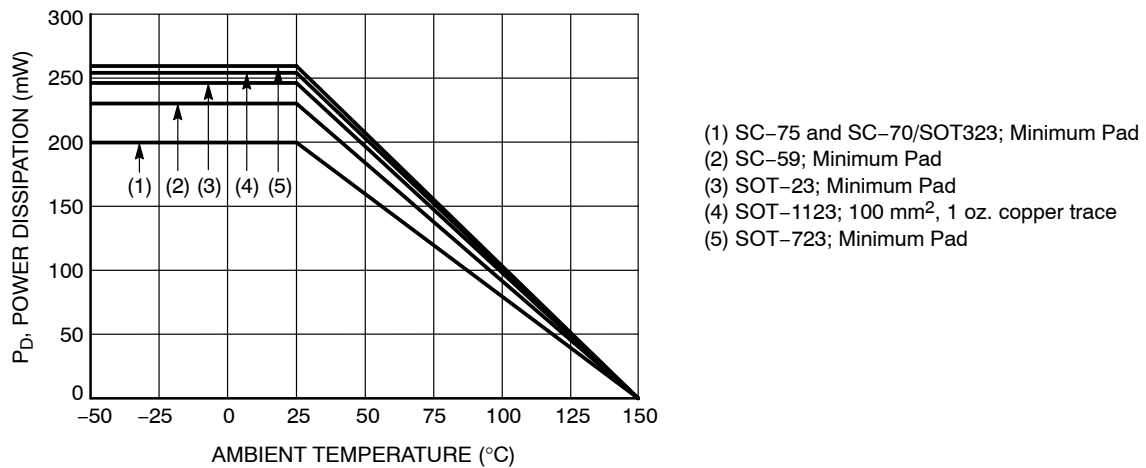
Figure 1. Derating Curve
