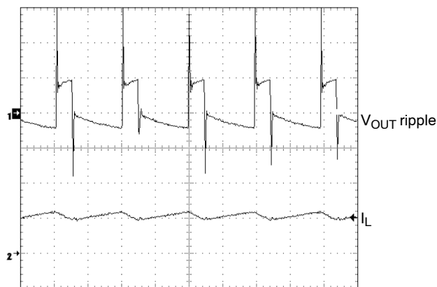
Figure 36. Typical Output Voltage Ripple
