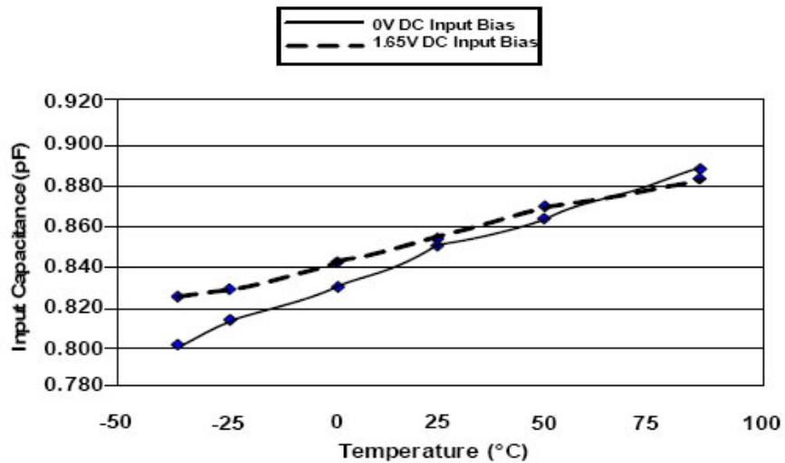
Figure 2. Typical Variation of C_{IN} vs. Temp ( f = 1\text{ MHz} , V_{IN} = 30\text{ mV} , V_P = 3.3\text{ V} , V_N = 0\text{ V} , 0.1\text{ }\mu\text{F} Chip Capacitor between V_P and V_N )
