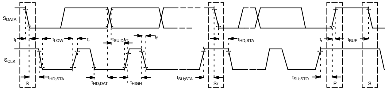
Figure 24. Master Two Wire Serial Bus Timing Parameters (CCIM)
