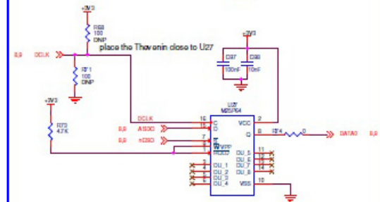
FPGA Memory I/F
