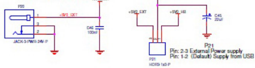
External +5V
