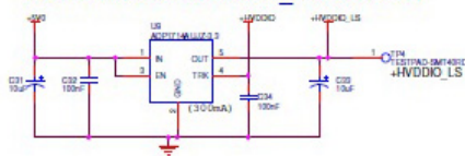
PERIPHERAL HVDDIO LS SUPPLY
