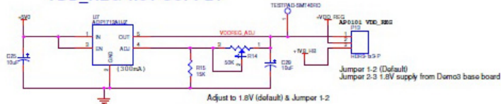
VDD REG 1.8V SUPPLY
