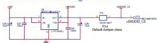
PERIPHERAL SVDDIO LS SUPPLY
