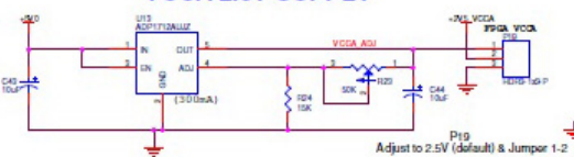
VCCA 2.5V SUPPLY
