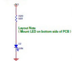
5V LED
