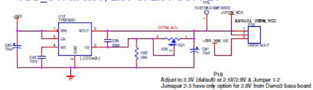
VDD_OTPM 3.3V, 2.8V or 2.5V SUPPLY
