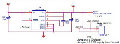
PERIPHERAL 3.3V SUPPLY
