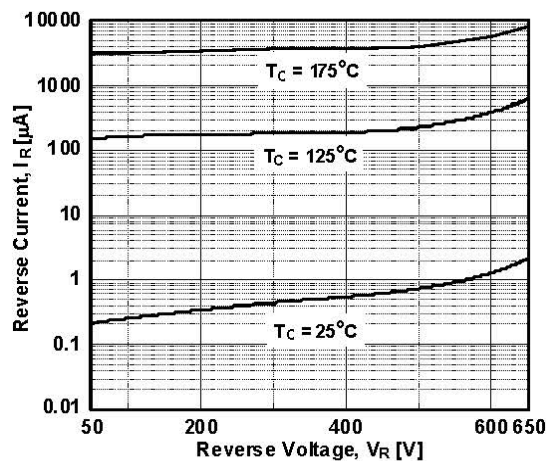
Figure 20. Reverse Current
