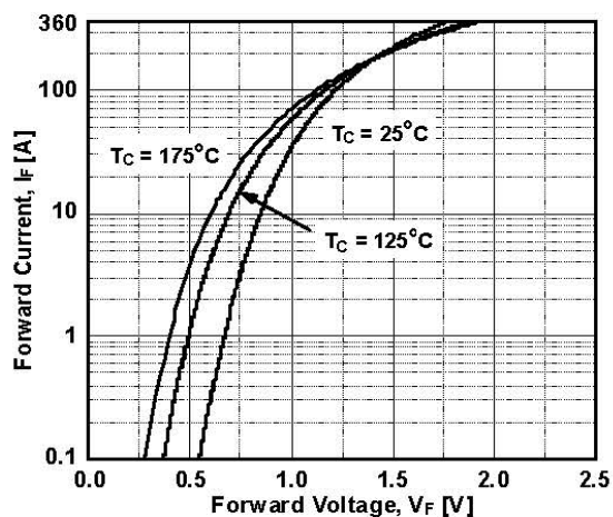
Figure 19. Forward Characteristics
