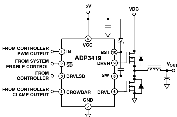
Figure 2. General Application Circuit
