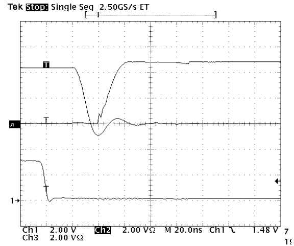
Figure 6. DRVH Fall and DRVL Rise Times CH1 = IN, CH2 = DRVH, CH3 = DRVL
