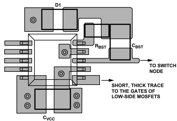
Figure 17. External Component Placement Example
