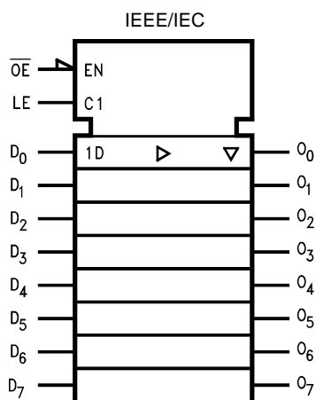
Figure 1. Logic Symbol
