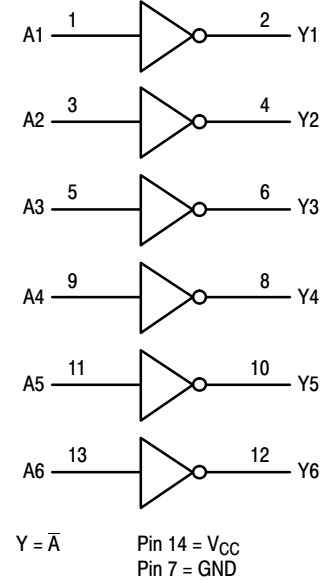
LOGIC DIAGRAM
