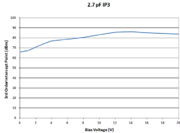
Figure 3. IP3*
