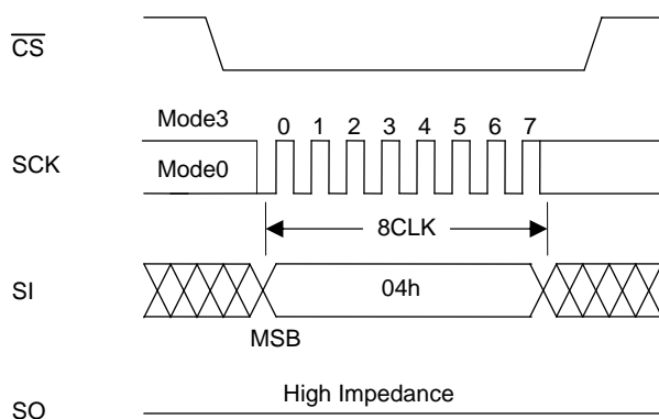
Figure 9. Write Disable
