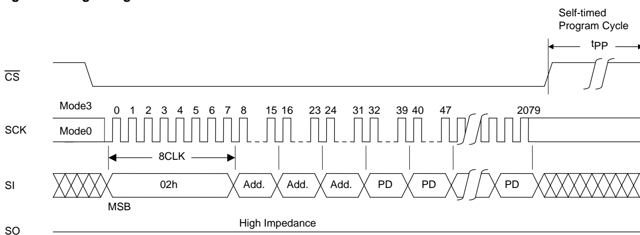
Figure 15. Page Program
