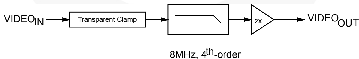
Figure 1. Block Diagram
