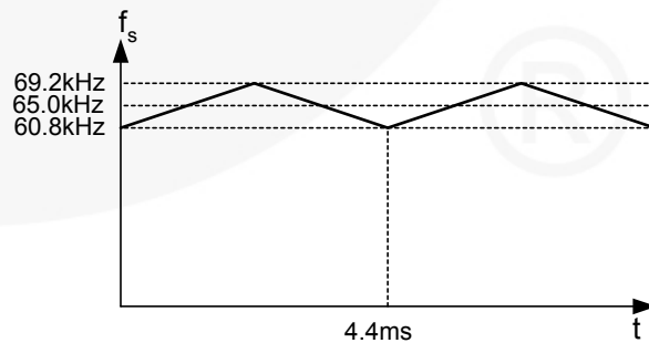
Figure 25. Frequency Hopping
