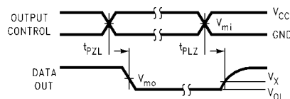
FIGURE 4. 3-STATE Output Low Enable and Disable Times for Low Voltage Logic t_R = t_F \leq 2.0 ns, 10% to 90%
