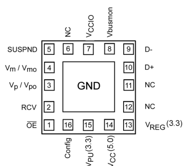
Figure 2. MLP16 GND Exposed Diepad (Bottom View)
