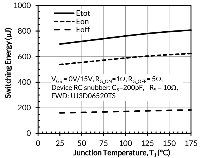
Figure 34. Clamped inductive switching energy vs. junction temperature at V_{\text{DS}} = 500\text{V} and I_{\text{D}} = 40\text{A}
