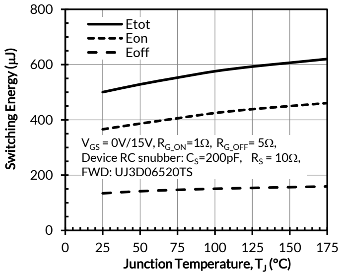
Figure 33. Clamped inductive switching energy vs. junction temperature at V_{\text{DS}} = 400\text{V} and I_{\text{D}} = 40\text{A}
