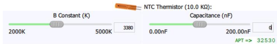
Figure 13. NTC THERMISTOR INPUT FEATURE
