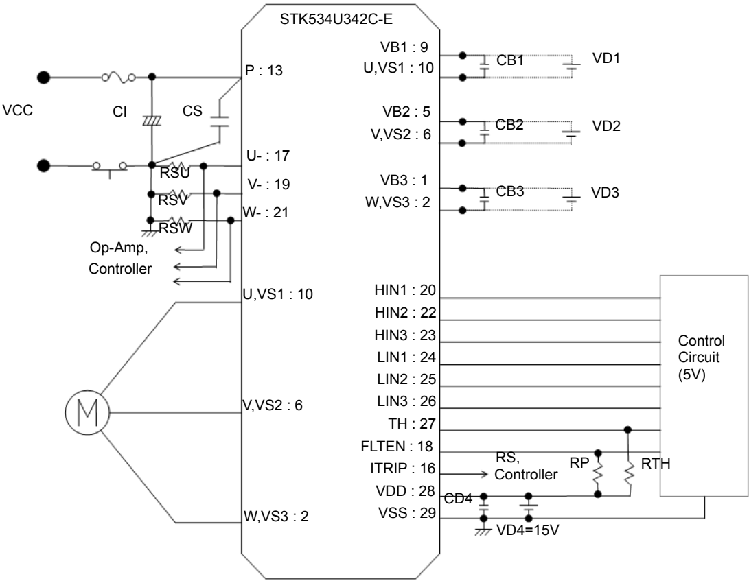
Sample Application Circuit
