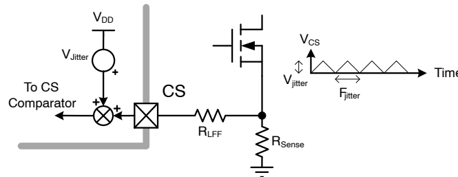
Figure 41. Frequency Jittering
