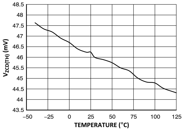
Figure 17. V ZCD(TH) vs. Junction Temperature
