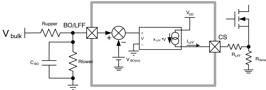
Figure 45. Internal Line Feed Forward Configuration V_{\text{CS(VCO)}} = 240 \text{ mV} and V_{\text{CS(STB)}} = 75 \text{ mV}
