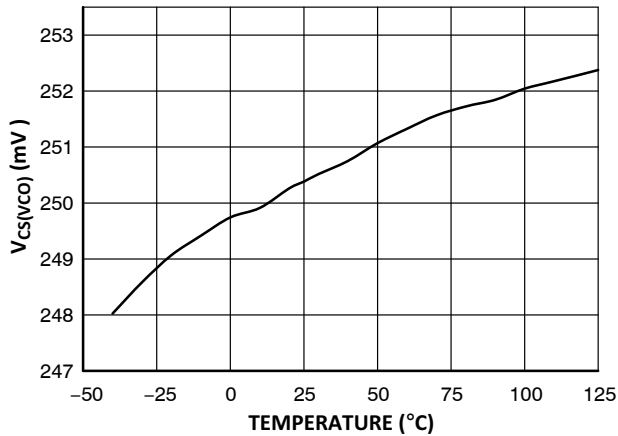
Figure 13. V CC(VCO) vs. Junction Temperature
