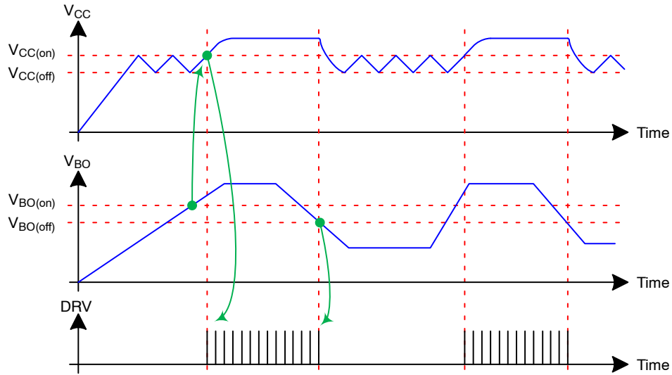
Figure 43. Brown-out Input Functionality – V_{CC} < V_{CC(on)}
