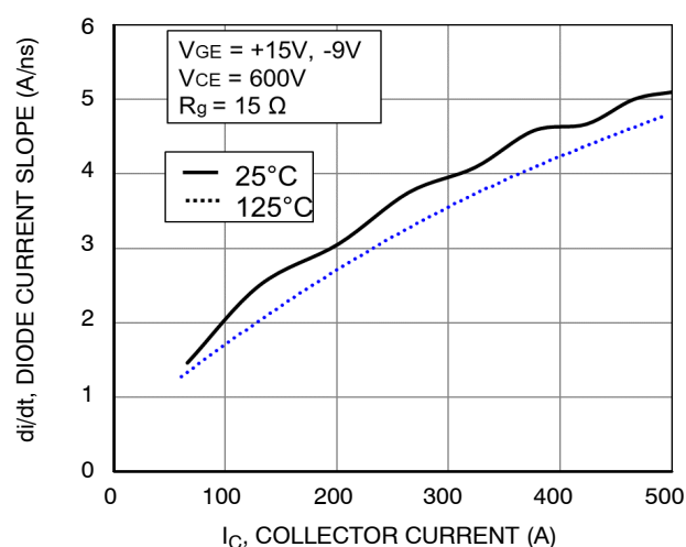
Figure 54. Typical di/dt vs. I_C
