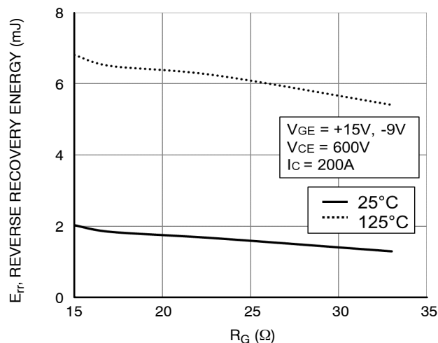
Figure 50. Typical Reverse Recovery Energy Loss vs. R_G
