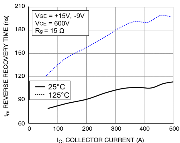
Figure 51. Typical Reverse Recovery Time vs. I_C
