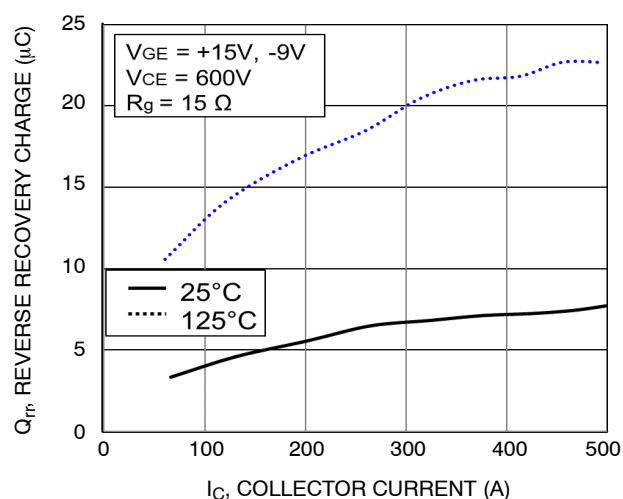
Figure 52. Typical Reverse Recovery Charge vs. I_C
