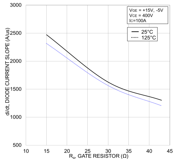
Figure 57. Typical di/dt vs. R_g
