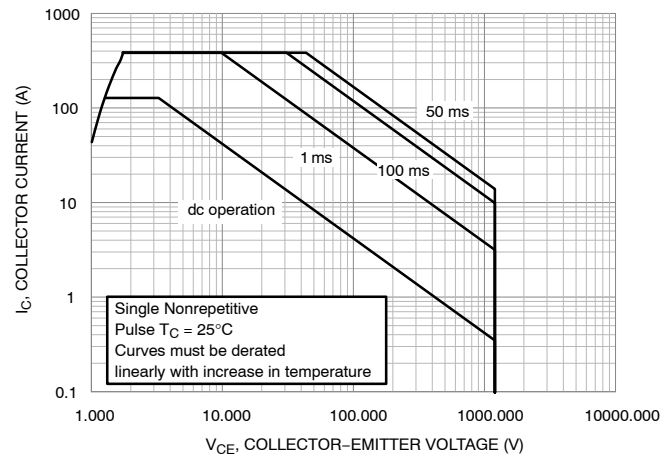
Figure 55. NP IGBT FBSOA
