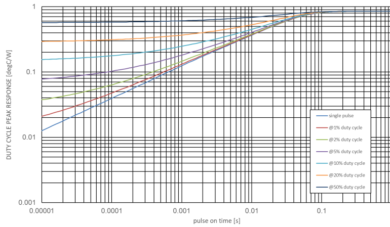
Figure 29. SiC MOSFET Junction-to-Case Transient Thermal Impedance
