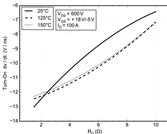
Figure 26. dv/dt ON vs. R_G
