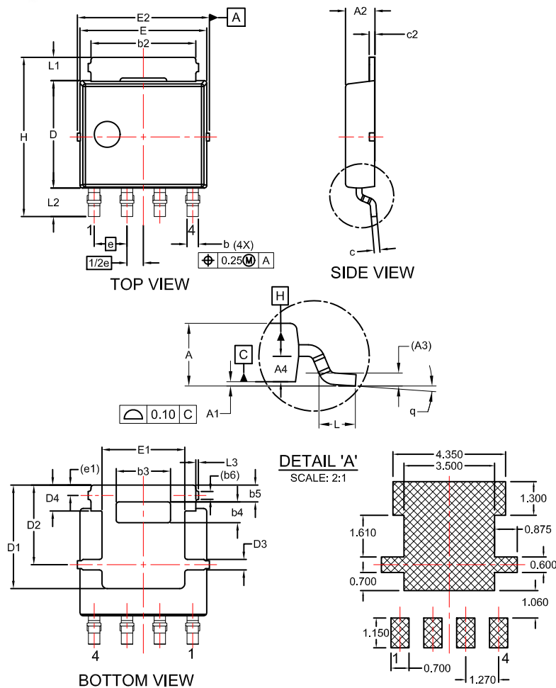
LFP4K4 5x6 CASE 760AB ISSUE C
