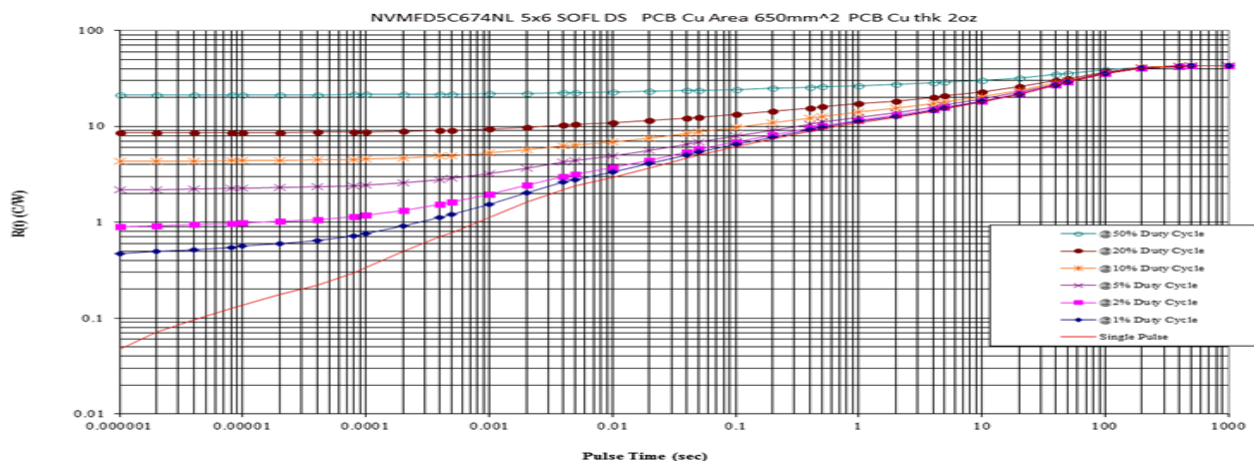
Figure 13. Thermal Characteristics
