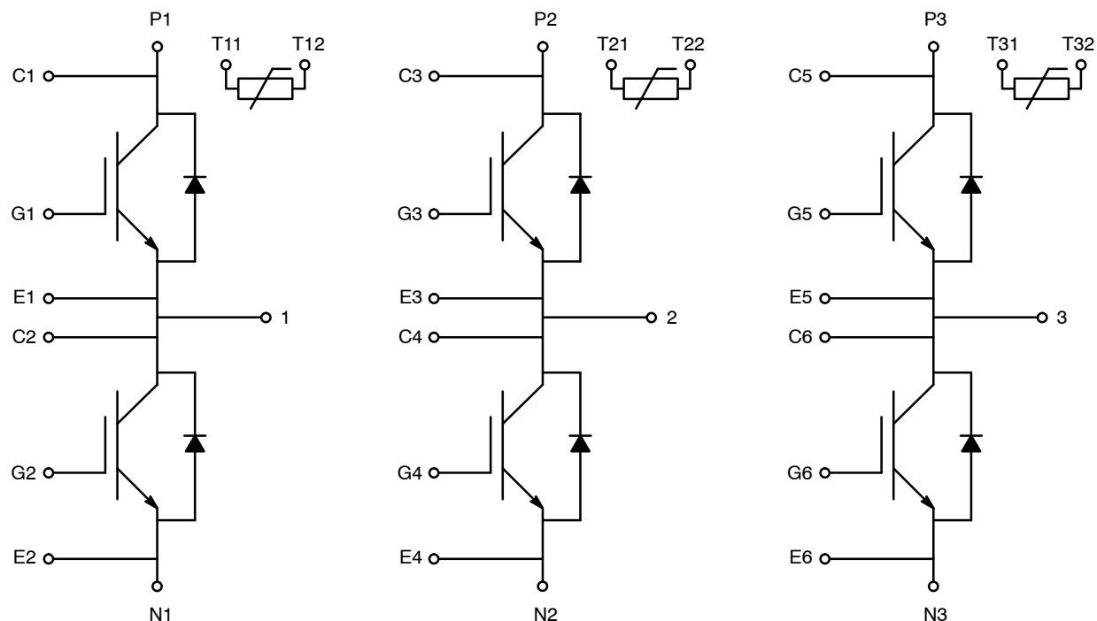
Figure 1. Pin Description
