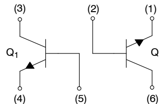
NST/NSV3904DXV6
