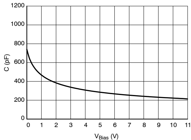
Figure 5. CV Characteristics
