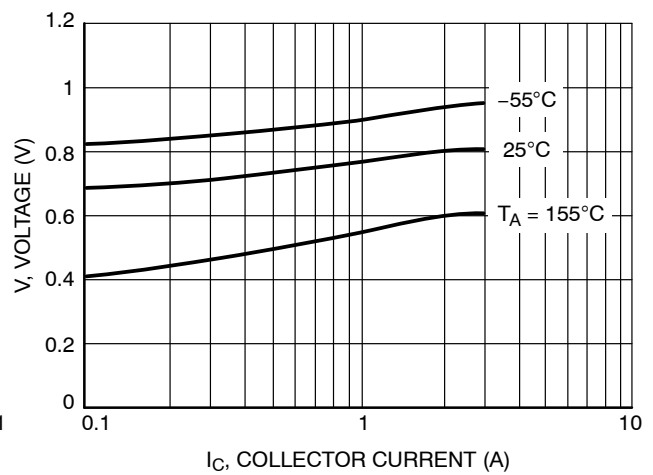
Figure 6. V_{BE(on)} Voltage
