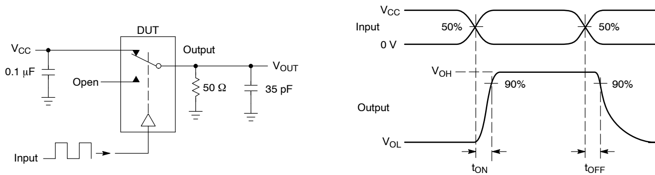
Figure 1. t_{ON}/t_{OFF}
