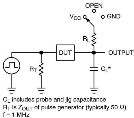
Figure 3. Test Circuit
