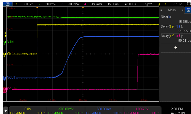
Figure 30. Turn-on Response
